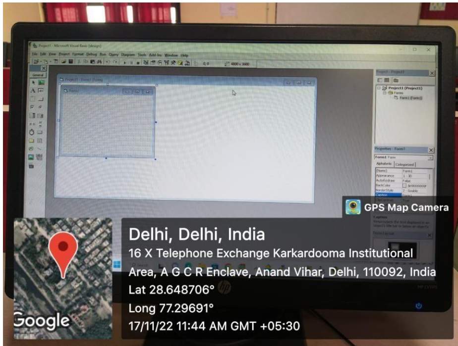
Visual Basic 6.0
