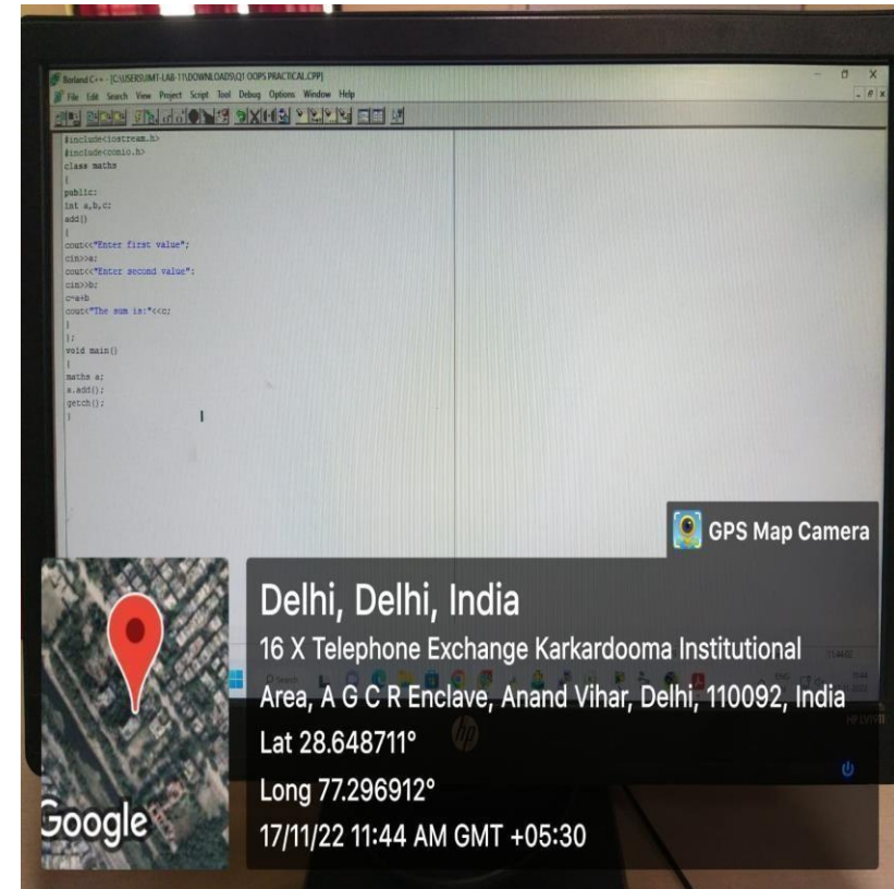
Borland C++
